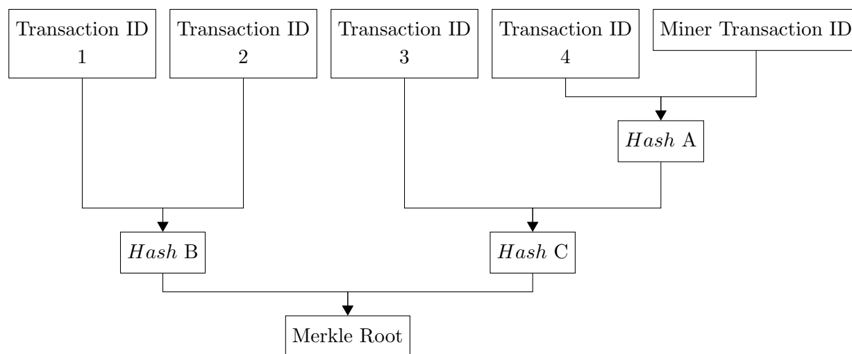
Figure 7.1: Merkle Tree
